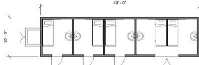
5 unit floor plan with individual sinks Cost per module: $102,950
