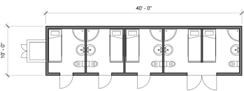
5 unit floor plan w/ individual showers, toilets, & sinks Cost per module: $130,550
